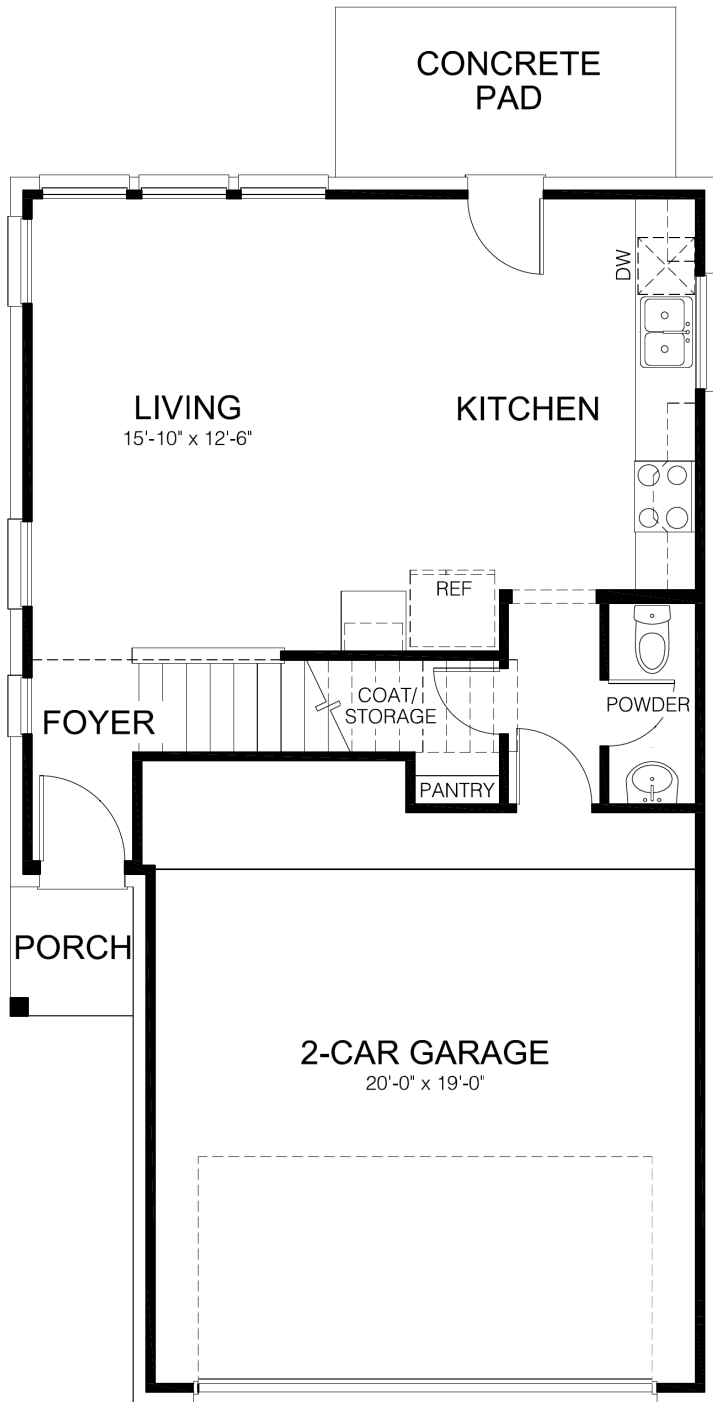
MAIN FLOOR PLAN ELEVATION A
