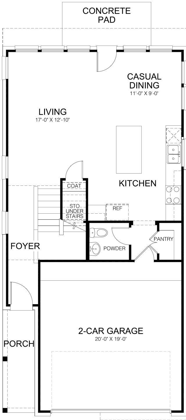
MAIN FLOOR PLAN ELEVATION A
