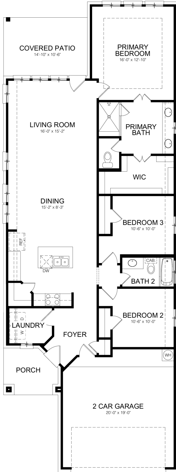
MAIN FLOOR PLAN ELEVATION A
