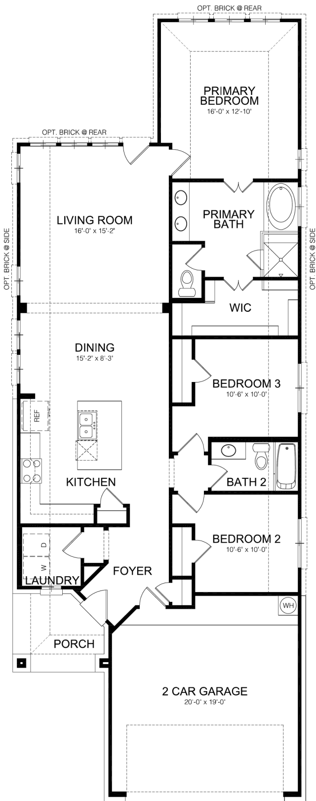
MAIN FLOOR PLAN ELEVATION A
