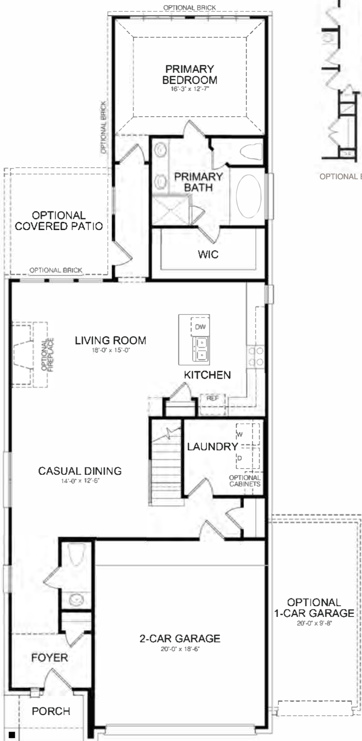
MAIN FLOOR PLAN ELEVATION A
