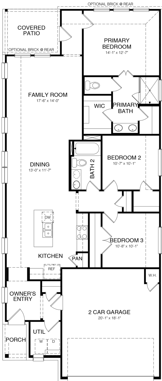
MAIN FLOOR PLAN STYLE A
