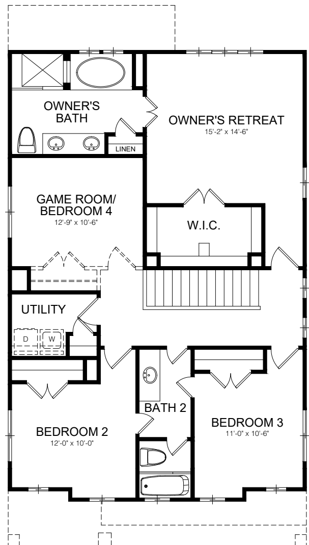
SECOND FLOOR PLAN STYLE D
