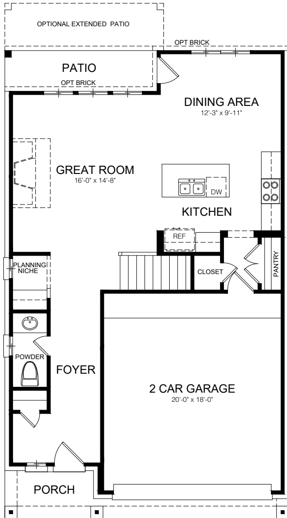
MAIN FLOOR PLAN STYLE D
