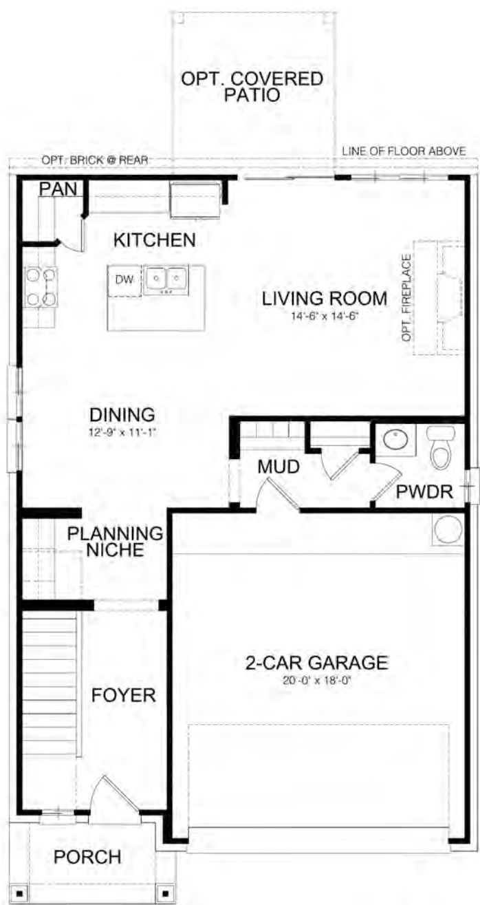
MAIN FLOOR PLAN ELEVATION B
