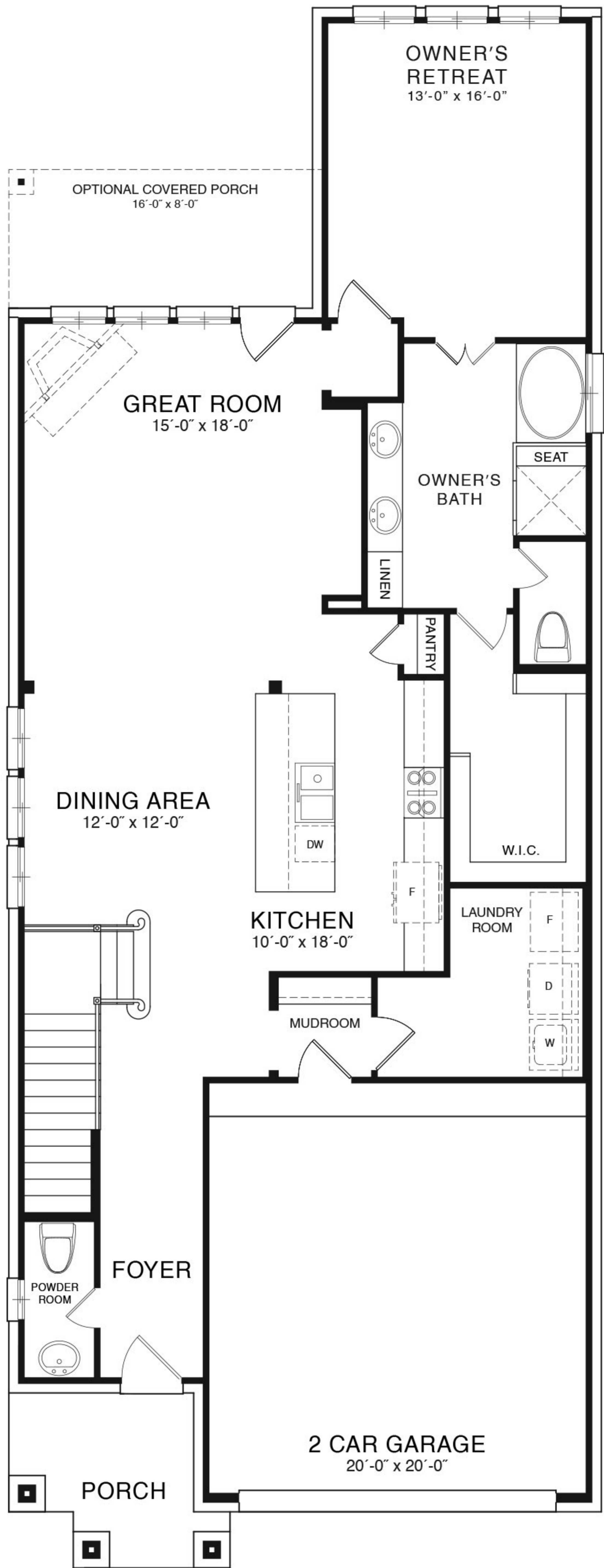
MAIN FLOOR PLAN STYLE A
